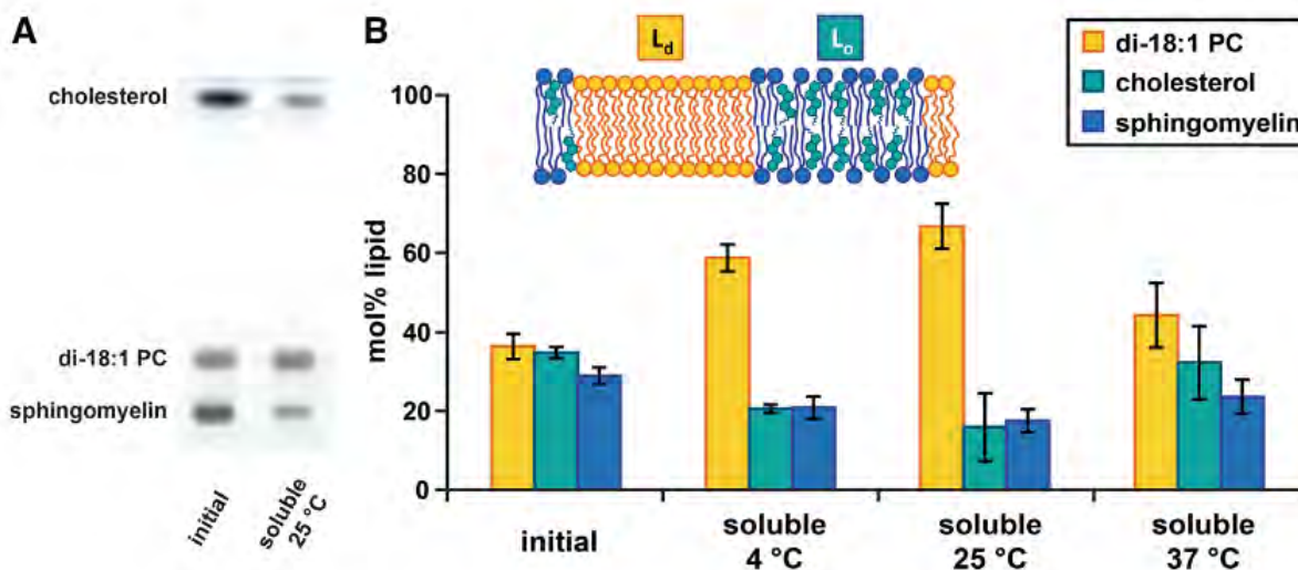
Figure 1-3 TLC for investigation of lipid incorporation into SMALPs. Figure reproduced from Dominguez-Pardo et al. Eur Biophys J. 2017.
