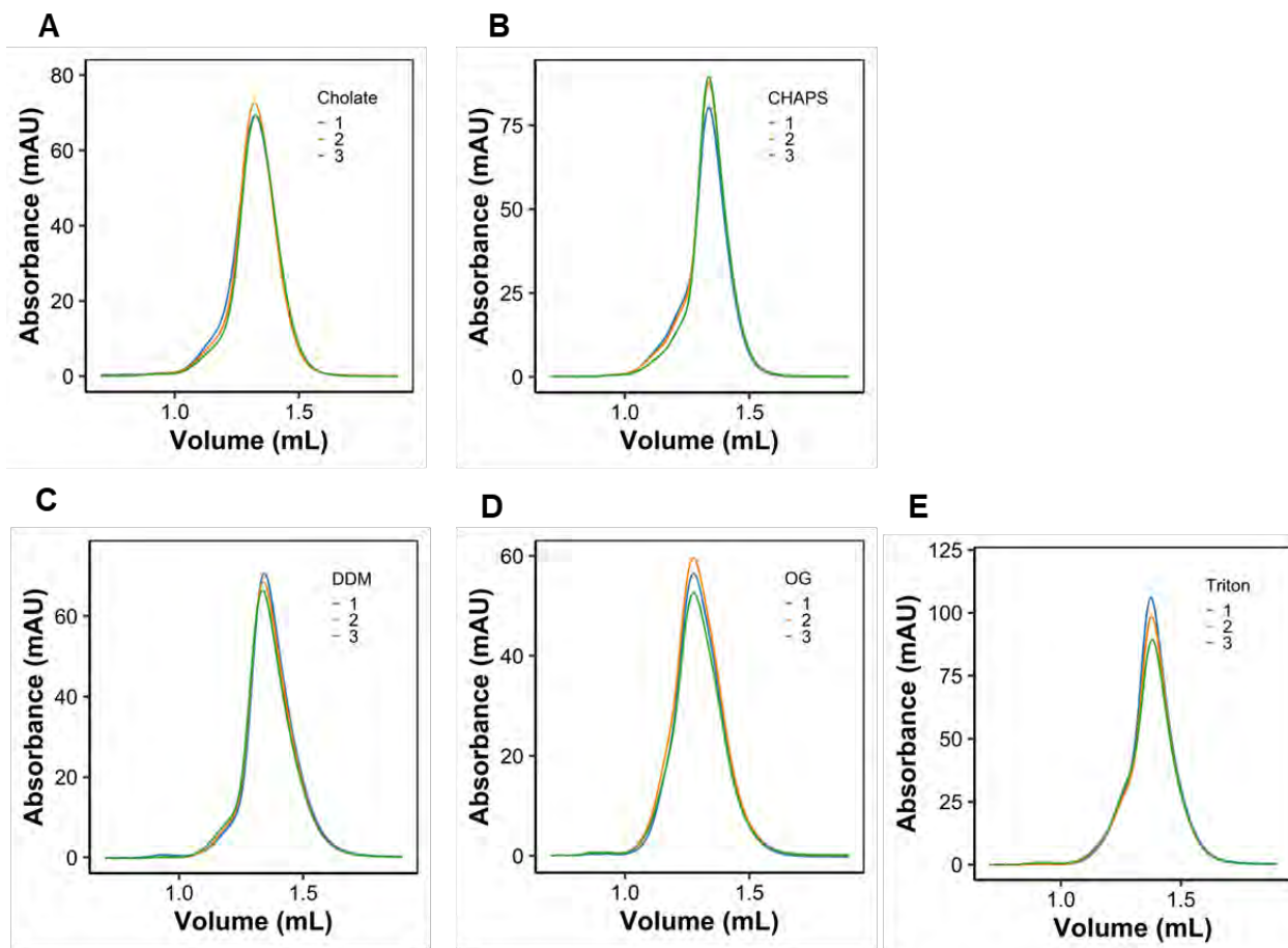
Figure A-IV-1 Representative size exclusion chromatograms of Nanodiscs synthesized with natural lipid extract mixtures and different detergents after SEC purification. Nanodiscs made with chololate (A), CHAPS (B), DDM (C), OG (D), and Triton X-100 (E).
